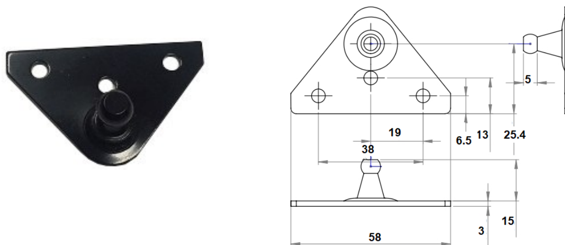
SF104B-3TK - Bracket with 10mm Ball Stud. Black Steel 3mm thick
