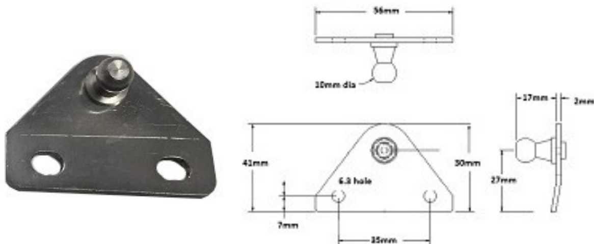
SF101S - Bracket with 10mm Ball Stud and Offset. Stainless Steel
