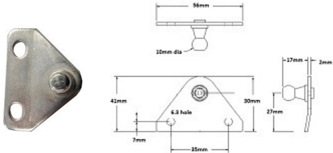
SF101S - Bracket with 10mm Ball Stud and Offset. Stainless Steel
